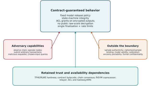
Figure 6: Security boundary and retained trust. Contract invariants cover the fixed release policy, state machine, ACL grants, raw-score non-publication, finalization, and rate limits under explicit infrastructure assumptions. Biological sample authenticity, ciphertext/sample binding, model validity, calibration, ancestry portability, and formal model confidentiality remain outside the boundary.
