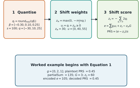
Overflow-safe unsigned fixed-point encoding Half-away-from-zero rounding and a clamped weight zero-point are part of the executable specification
