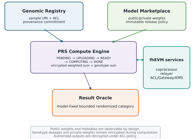
bioETH-PRS system architecture Four contracts orchestrate policy while fhEVM services execute encrypted operations
